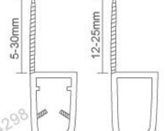
RL-WS-007G
