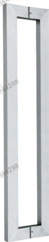
RL-DH028 Size(mm) A:1000 B:962 D:φ38x25 A:1200 B:1062 D:φ38x25 Colour:Chrome plate /Stain nickel
