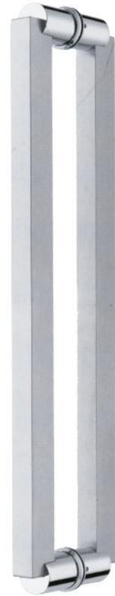
RL-DH026 Size(mm) A:600 B:400 D:φ38x19 Colour:Chrome plate /Stain nickel
