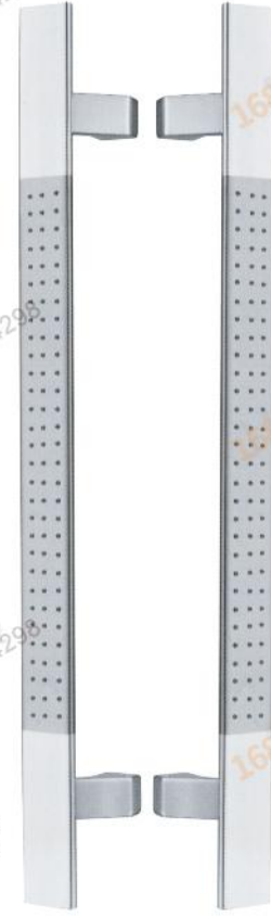
RL-DH028 Size(mm) A:1000 B:962 D:φ38x25 A:1200 B:1062 D:φ38x25 Colour:Chrome plate /Stain nickel
